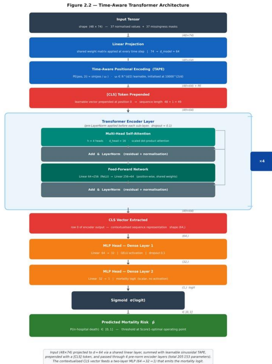
Figure 2.2 – Schematic of the Time-Aware Transformer
