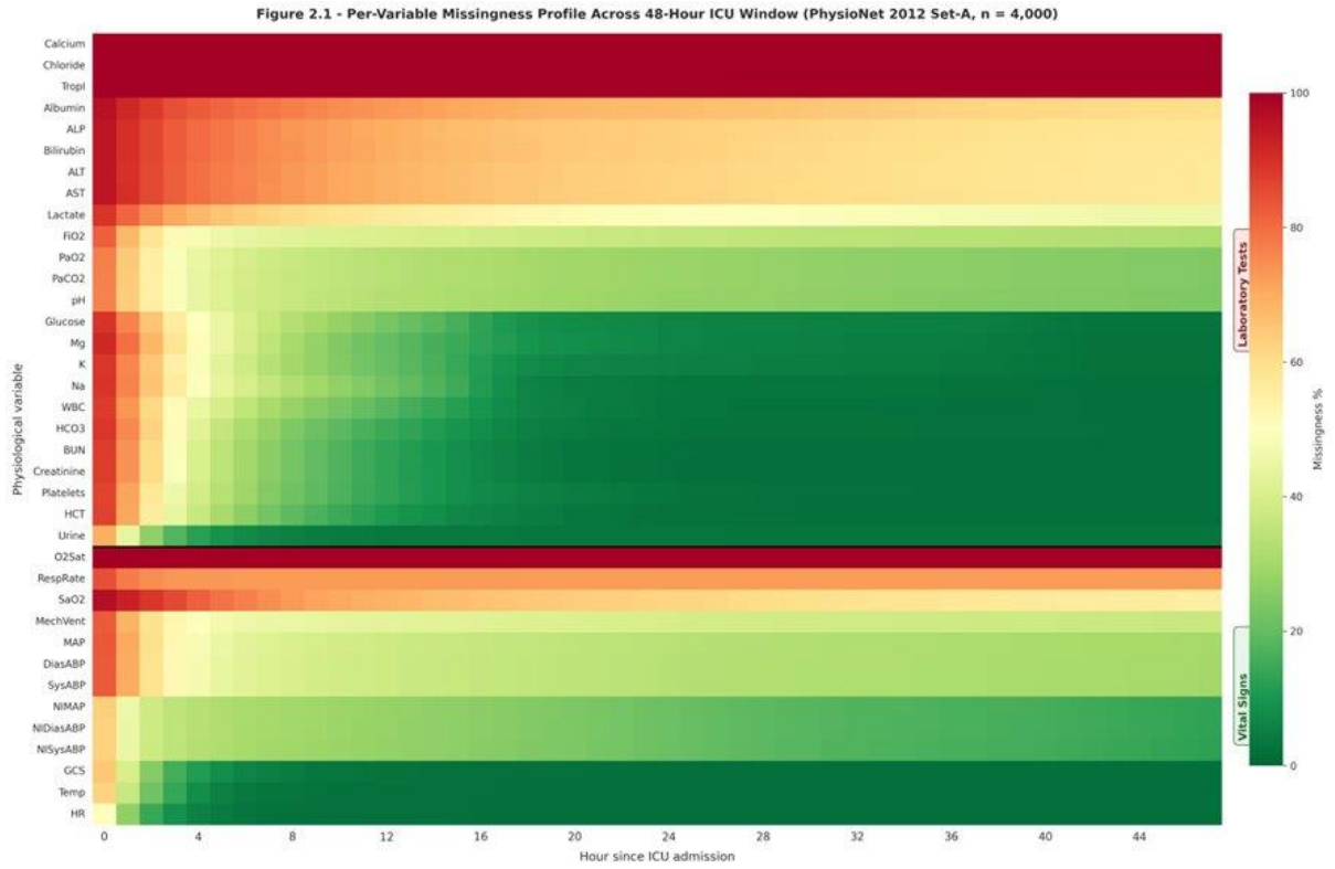
Figure 2.1 – Per-variable missingness profile across the 48-hour window of the PhysioNet 2012 Set-A cohort
