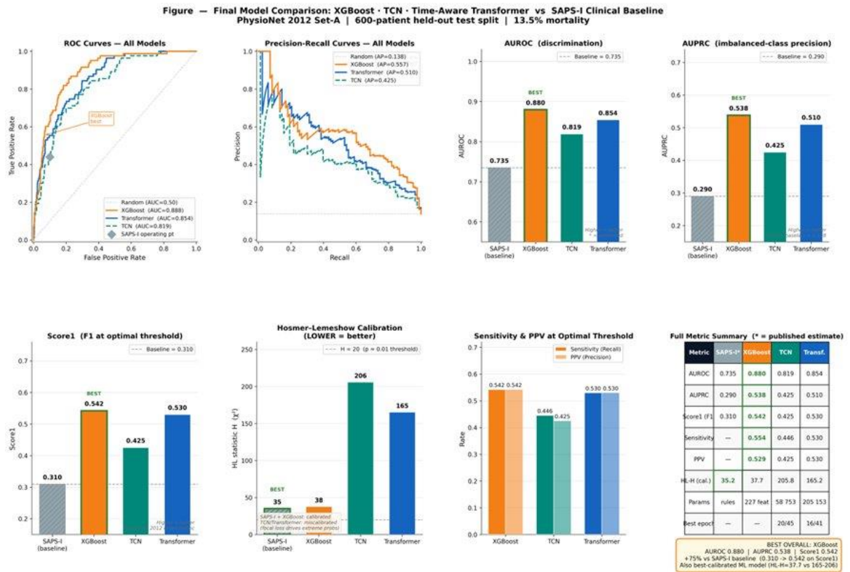
Figure 3.3 – Final comparison of the four predictors across the discrimination and balance metrics
